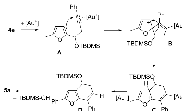
Scheme 3. Proposed mechanism for the gold(I)-catalyzed rearrangement of the substrate 4a to the 2,7-disubstituted benzo[ b ]furan 5a .
