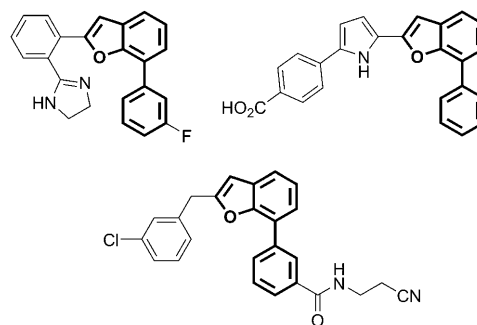
Scheme 2. Bioactive compounds with a 7-aryl benzofuran core structure. [9]
