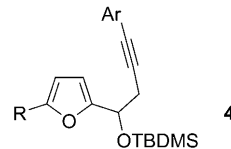
Figure 1. Furan derivatives 4 are structurally related to Kirsch's substrate 1 . Ar = aryl, hetaryl; R = alkyl, aryl; TBDMS = tert -butyldimethylsilyl.
