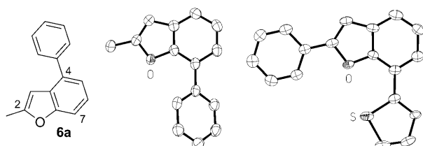
Figure 2. Left: Conceivable structure of benzofuran 6a . Middle: Solid-state molecular structure of 5a . Right: Solid-state molecular structure of the sulfur-containing product 5i . Thermal ellipsoids at 50 % probability.
