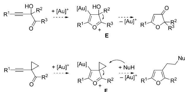
Scheme 4. Furan-derived Wheland-type intermediates according to Kirsch et al. and Schmalz and co-workers. Top: R 1 = aryl, alkyl; R 2 = alkyl; R 3 = aryl, alkyl; bottom: R 1 = aryl, alkyl; R 2 = aryl, alkyl; Nu = R 3 O.
