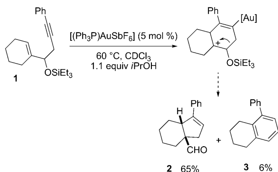
Scheme 1. Gold-catalyzed cyclization/pinacol rearrangement and the competing reaction according to Kirsch et al.
